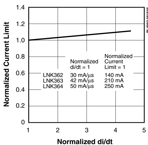
Figure 13. Current Limit vs. di/dt .
