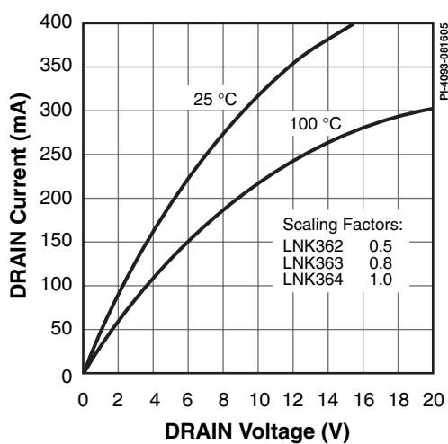
Figure 15. Output Characteristics.
