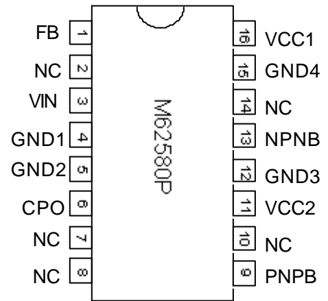
Outline 16P4
