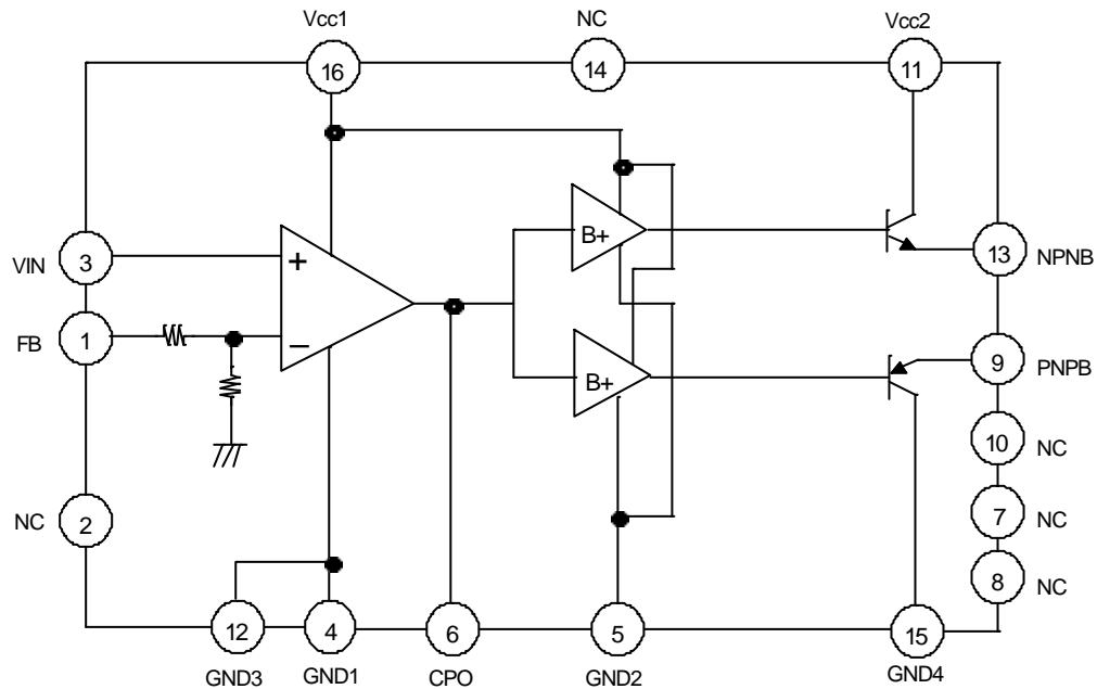
BLOCK DIAGRAM
