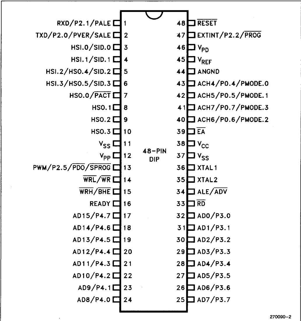
Figure 10. 48-Pin DIP Package
