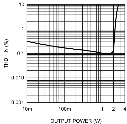
THD+N vs Output Power V_{DD} = 5V , R_L = 3\Omega
