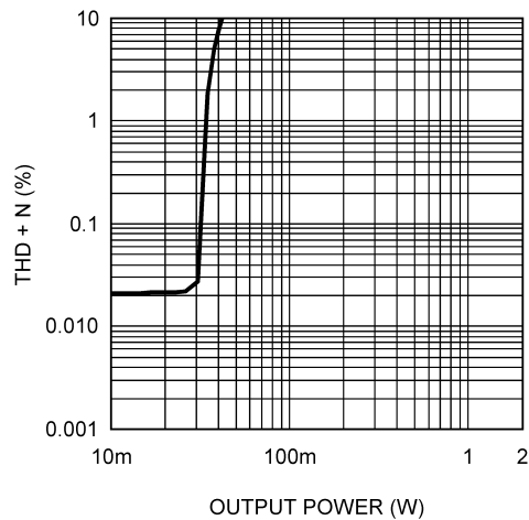
THD+N vs Output Power V_{DD} = 3V , R_L = 32\Omega , SE
