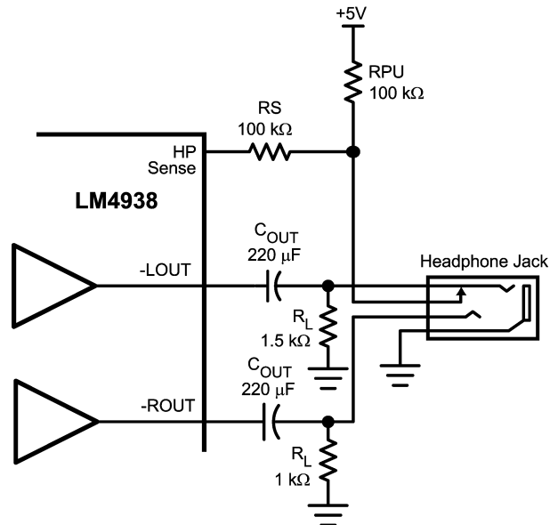
FIGURE 3. Headphone Sensing Circuit
