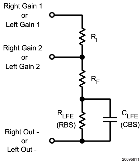
FIGURE 4. Low Frequency Enhancement
