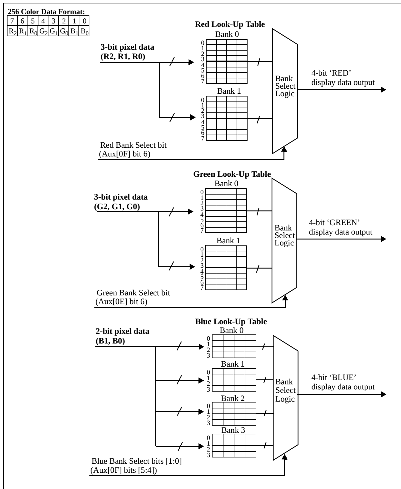
Figure 9: 256-Level Color Mode Look-Up Table Architecture
