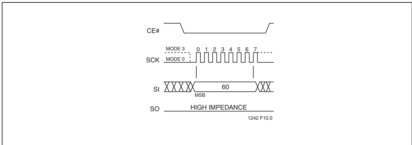
FIGURE 10: CHIP-ERASE SEQUENCE
