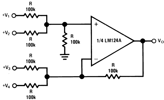
DC Summing Amplifier (V_{\text{IN}'\text{'S}} \geq 0\text{ V}_{\text{DC}} \text{ and } V_{\text{O}} \geq V_{\text{DC}})
