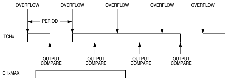
Figure 11-11. CHxMAX Latency
