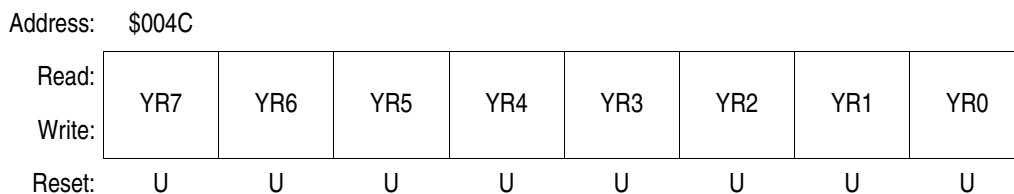
Figure 12-18. Year Register (YRR)
