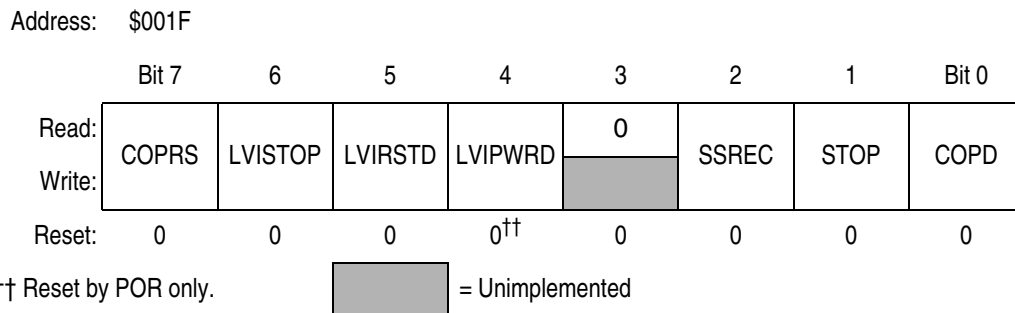
Figure 21-2. Configuration Register 1 (CONFIG1)
