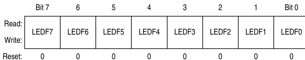
Figure 18-23. Port F LED Control Register (LEDF)
