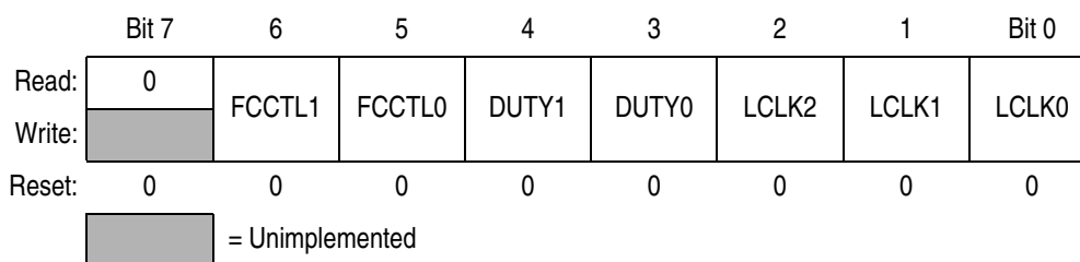
Figure 17-17. LCD Clock Register (LCDCLK)
