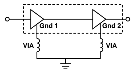
Figure 13. INA-34063 Suggested Layout.
