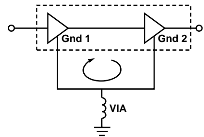
Figure 12. INA-34063 Potential Ground Loop.
