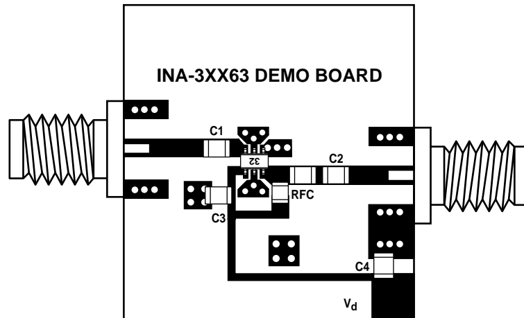
Figure 14. Assembled Amplifier.
