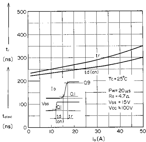
Turn-ON Characteristics
