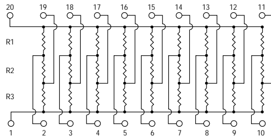
830 ELECTRICAL SCHEMATIC
