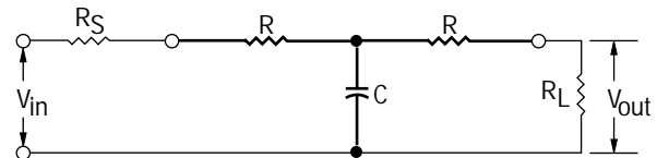
Figure 2. basic T-Filter configuration
