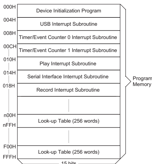
Program Memory
