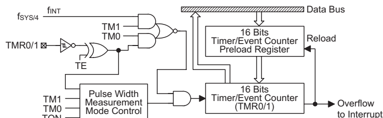
Timer/Event Counter 0/1
