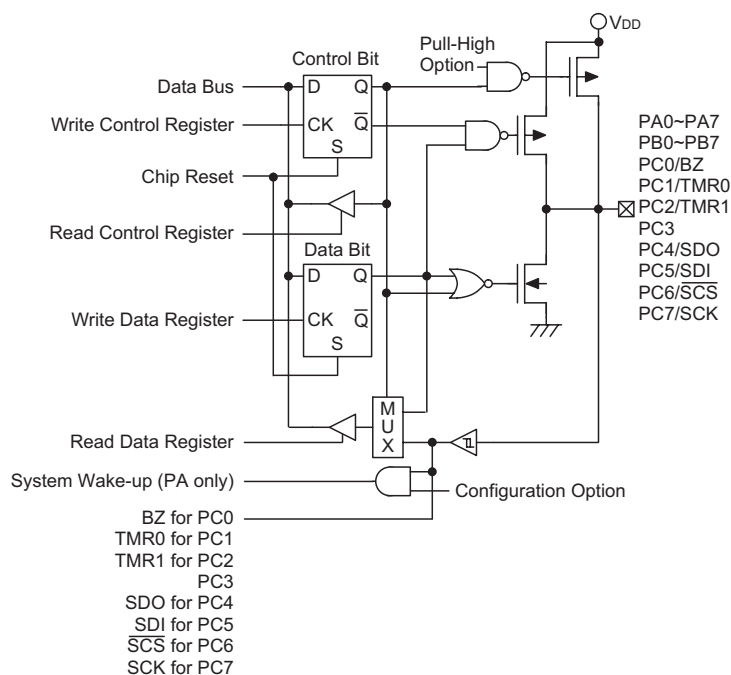
Input/Output Ports
