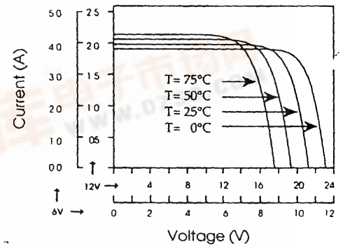
VLX - 32 IV-CHARACTERISTICS
