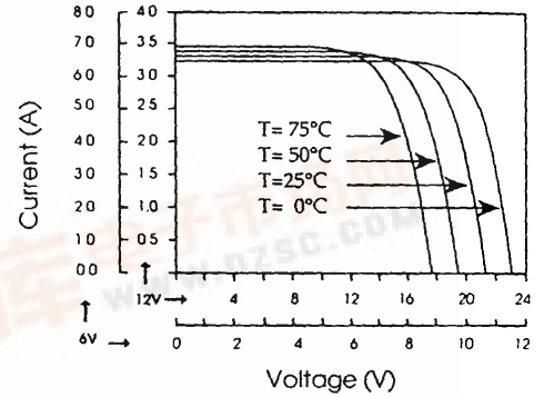
VLX - 53 IV-CHARACTERISTICS
