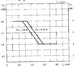
Fig. 12 - Sending and receiving gain vs. line current
