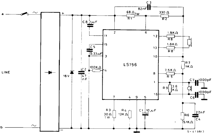
Fig. 11 - Application circuit without multifrequency.
