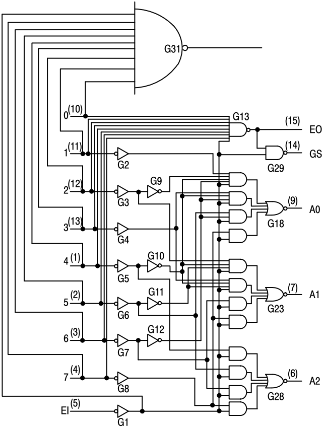
SN54/74LS748
