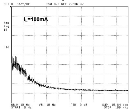
Output Noise
