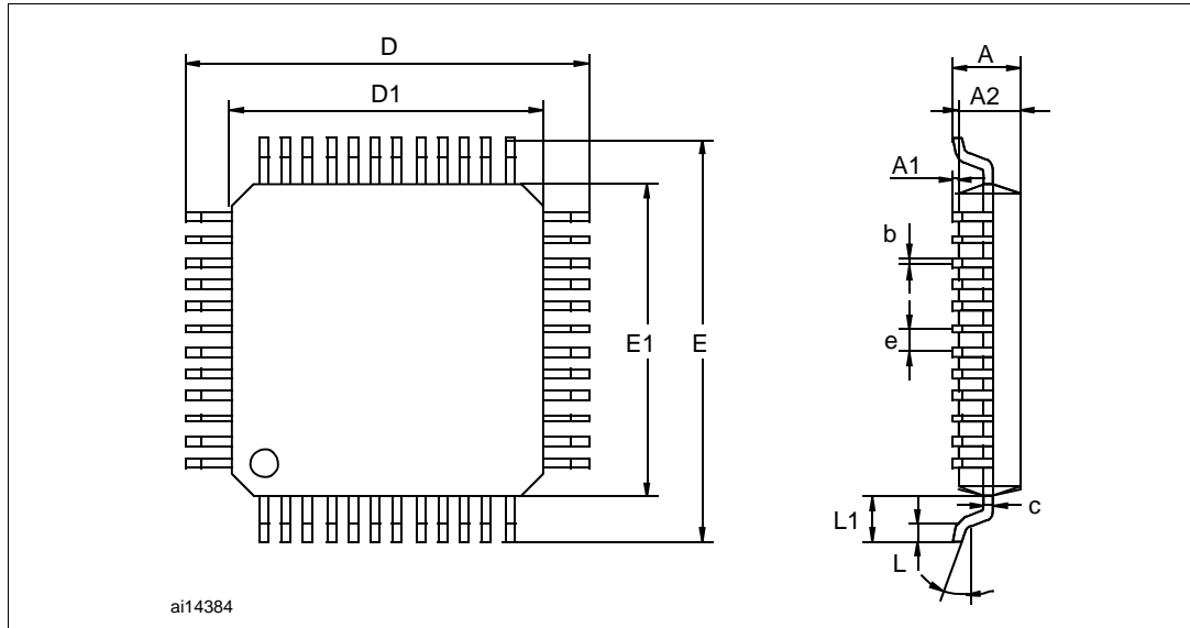
Figure 27. LQFP48 – 48-pin low-profile quad flat package outline
