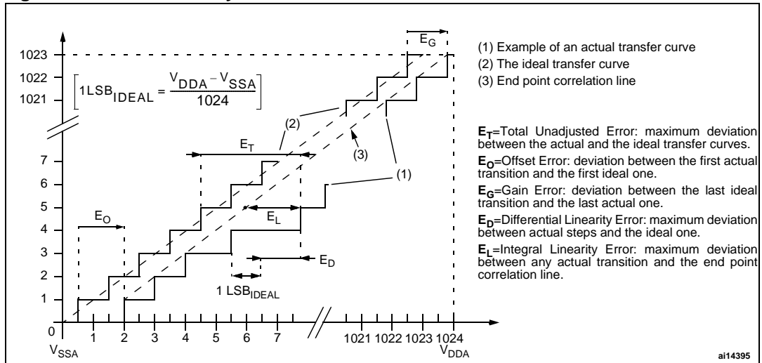
Figure 21. ADC accuracy characteristics
