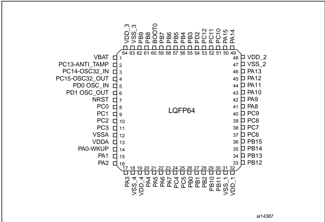
Figure 3. STM32F101xx access line LQFP64 pinout
