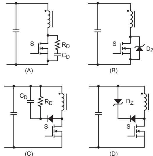
Figure 5—Snubber Designs
