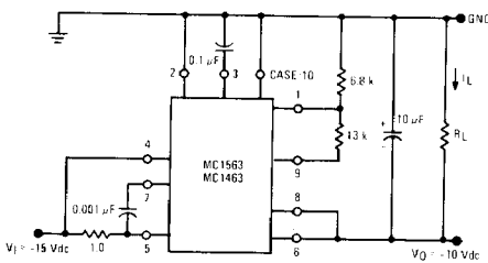
FIGURE 8 - SHUTDOWN CURRENT
