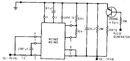
FIGURE 7 - OUTPUT IMPEDANCE
