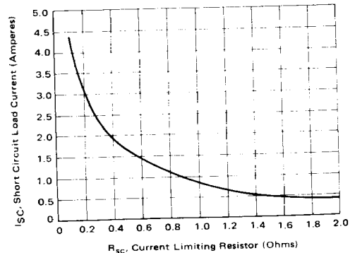
FIGURE 27 — I_{SC} versus R_{SC} (REFERENCE FIGURE 26)
