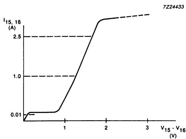
Fig.11 Saturation curve.
