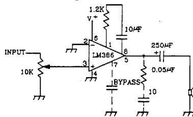
Amplifier 2
