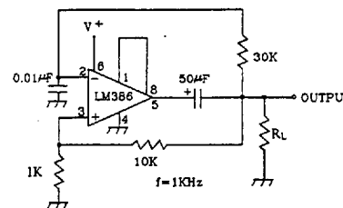
Square Wave Oscillator
