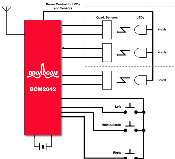
BCM2042 Mouse Block Diagram
