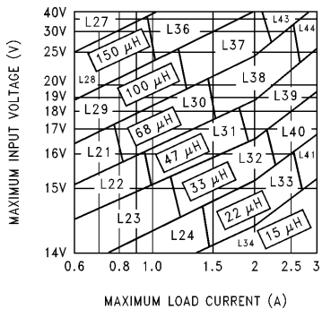
FIGURE 7. LM2596-12
