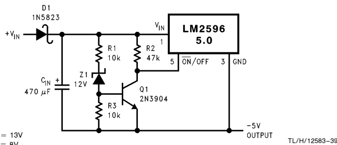
FIGURE 24. Undervoltage Lockout with Hysteresis for Inverting Regulator
