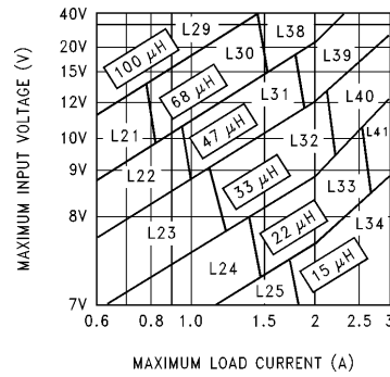
FIGURE 6. LM2596-5.0
