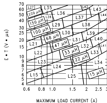
FIGURE 8. LM2596-ADJ
