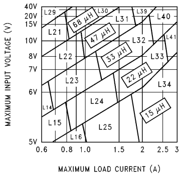
FIGURE 5. LM2596-3.3
