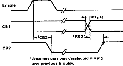
FIGURE 12 - CB2 DELAY TIME (Write Mode; CRB-5=1, CRB-3=CRB-4=0)
