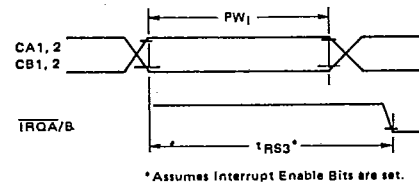
FIGURE 13 - INTERRUPT PULSE WIDTH AND \overline{IRQ} RESPONSE
