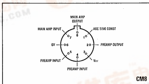
Fig.1 Pin connections, SL6270 - CM (bottom view)
