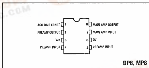
Fig.2 Pin connects, SL6270 - DP (top view)
