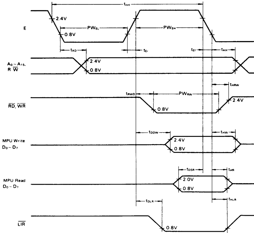
Figure 1 Bus Timing
