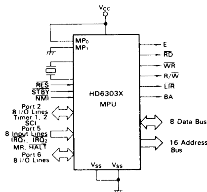
Figure 15 Operation Mode
