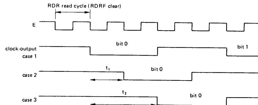
Precaution 1 Diagram
