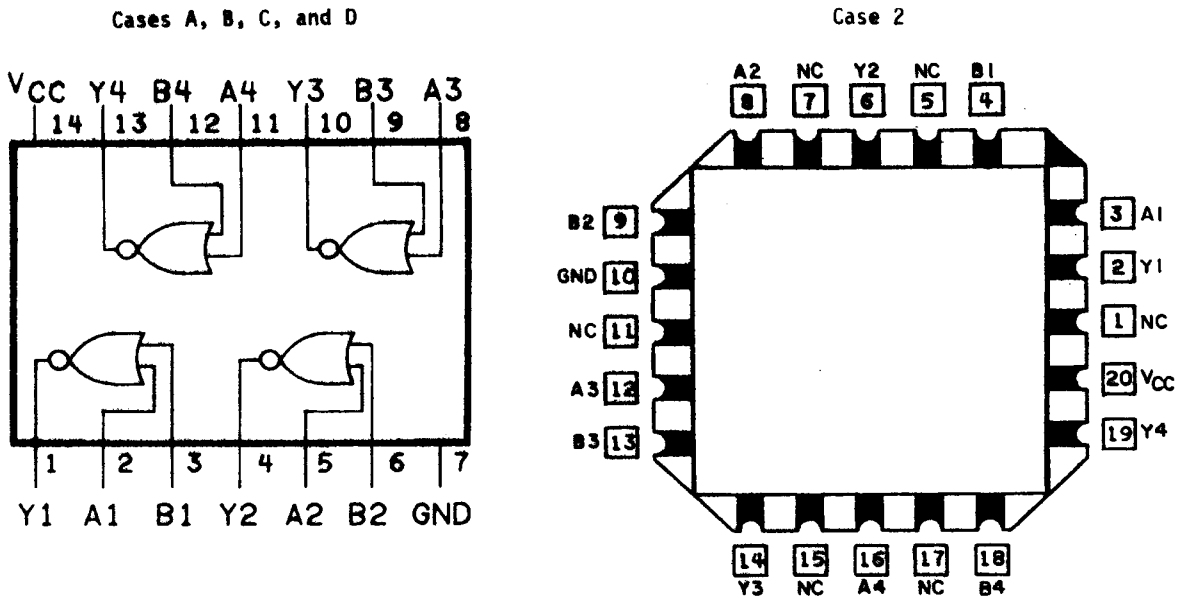
FIGURE 1. Terminal connections (top view).
