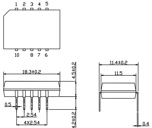
K (DIP10K)
