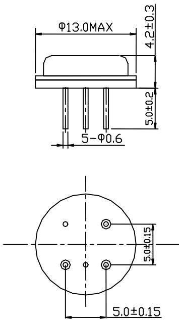
A (TO-5)
