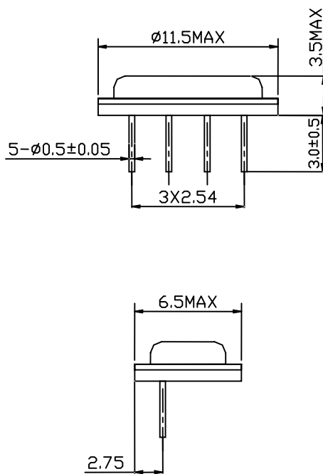
S (F-12)
