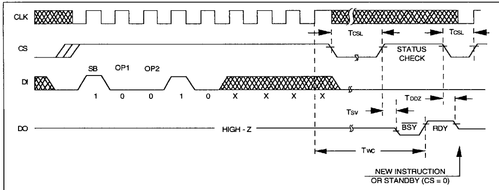
FIGURE 3-5: ERASE ALL
