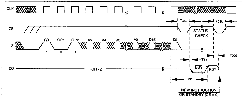
FIGURE 3-2: WRITE MODE
