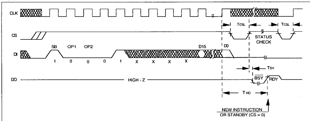
FIGURE 3-6: WRITE ALL
