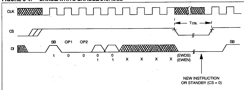
FIGURE 3-4: ERASE/WRITE ENABLE/DISABLE
