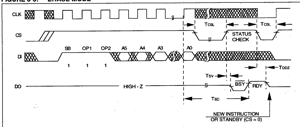
FIGURE 3-3: ERASE MODE
