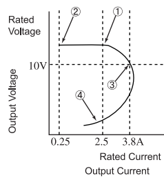
Fig1. Output Voltage/Current
