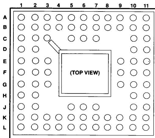
I/O Pin Assignments for the 84-Pin Ceramic Pin Grid Array Package
