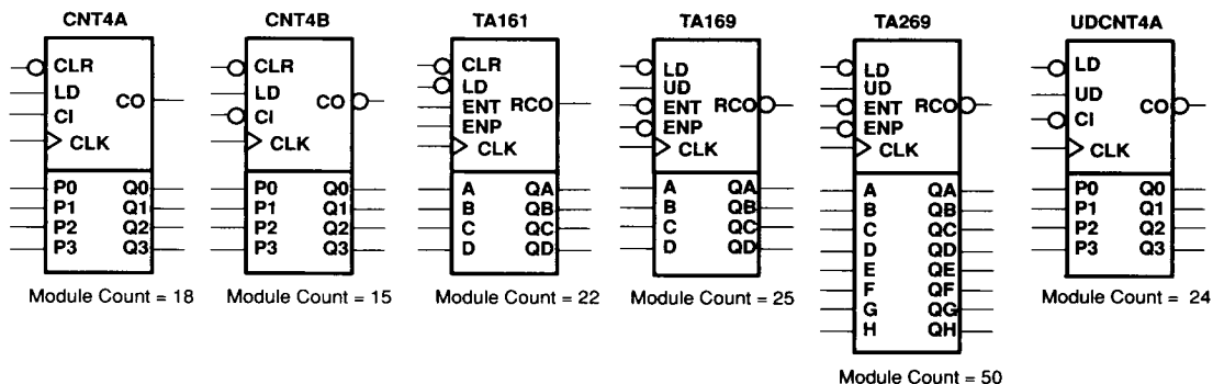
Figure 30. Counters
