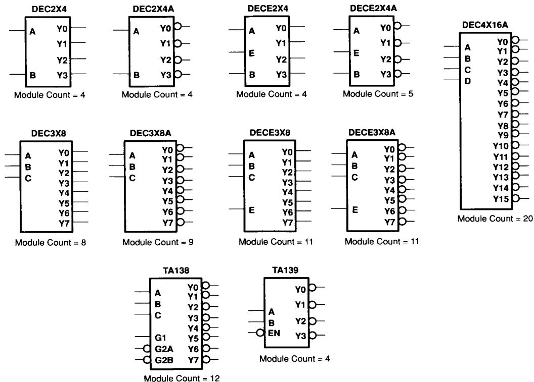
Figure 31. Decoders
