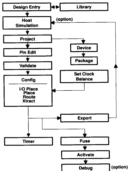
Figure 1. Design Flow
