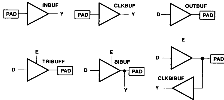
Figure 19. I/O Buffers
