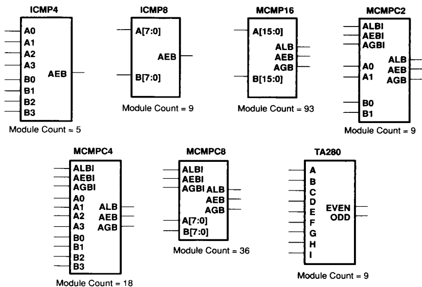
Figure 29. Comparators/Parity Checker
