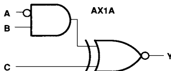
Figure 15. AND-XOR/AND-XNOR Gates
