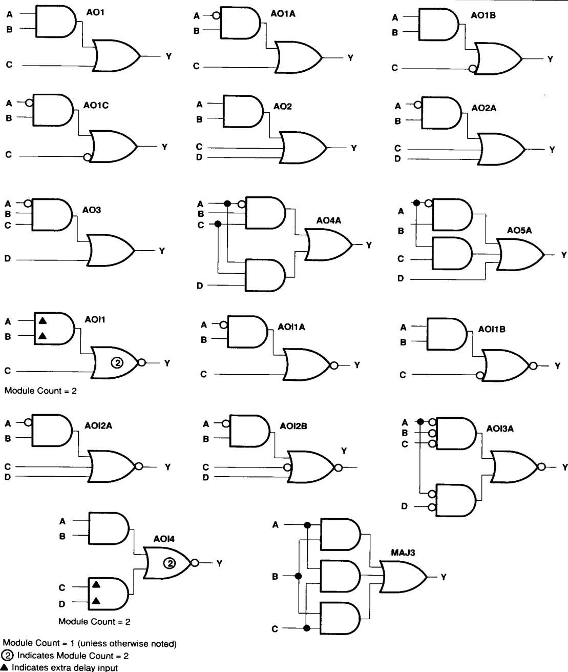
Figure 16. AND-OR/AND-NOR Gates
