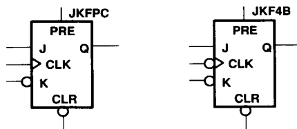
Figure 25. J-K Flip-Flops
