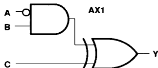
Figure 12. XOR/XNOR Gates
