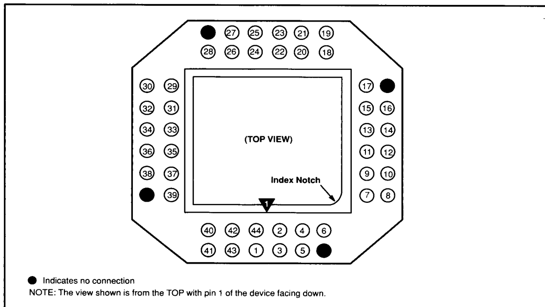
Figure 43. 44-Pin PLCC Actionprobe
