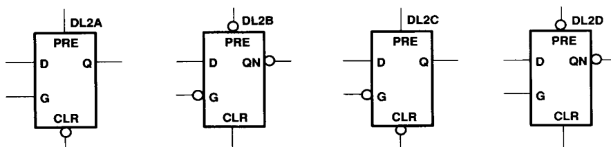
Figure 22. D-Type Latches
