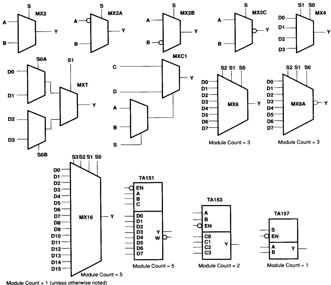
Figure 20. Multiplexers
