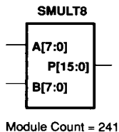
Figure 33. 8-Bit Multiplier
