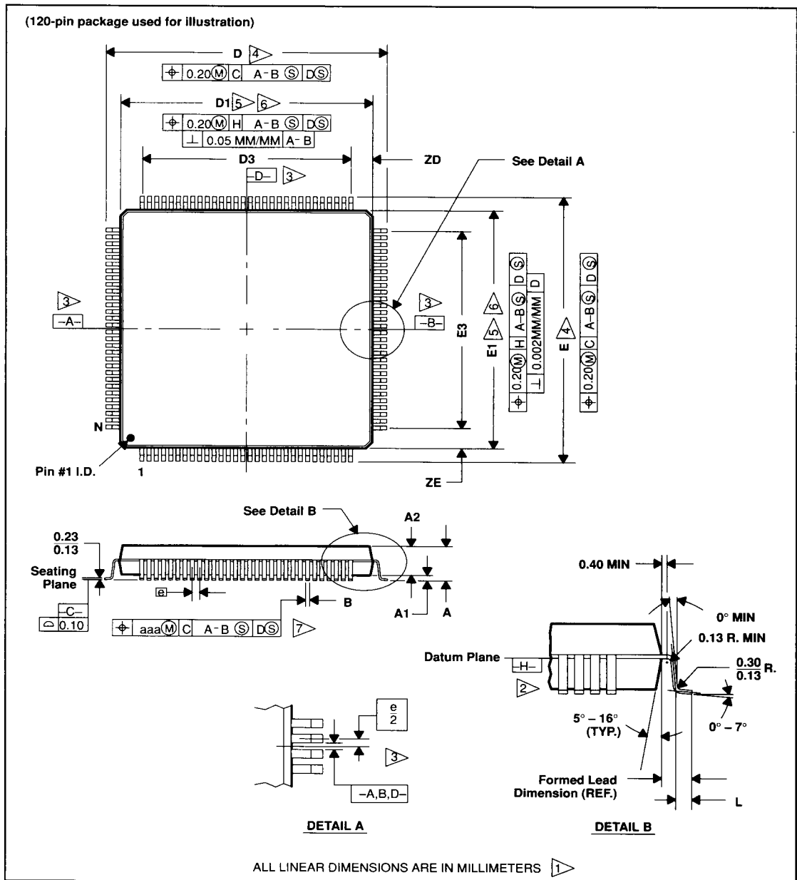
Figure 51. Plastic Quad Flat Packages
