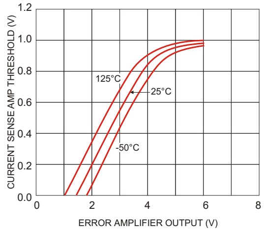
Figure 4. Current Sense Amplifier vs. Error Amplifier Output
