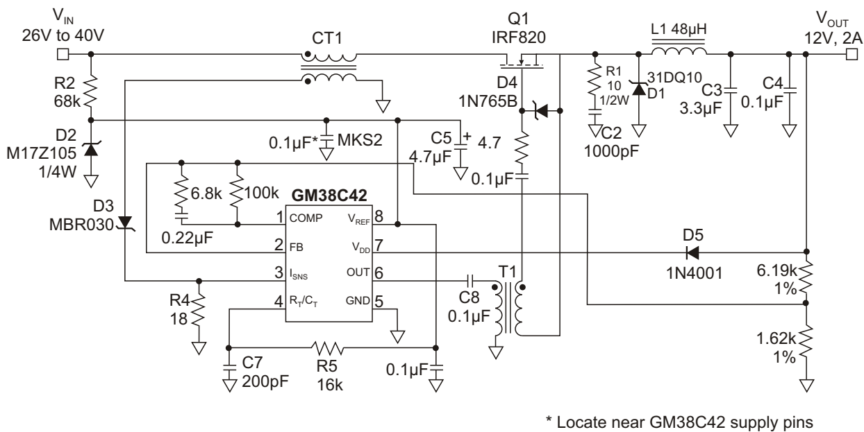
Figure 7. 500kHz, 25W, Buck Converter
