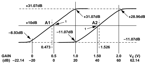
Figure 38. AD603 Gain Control Input Calculations for Sequential Operation V_C = 2.0\text{ V}
