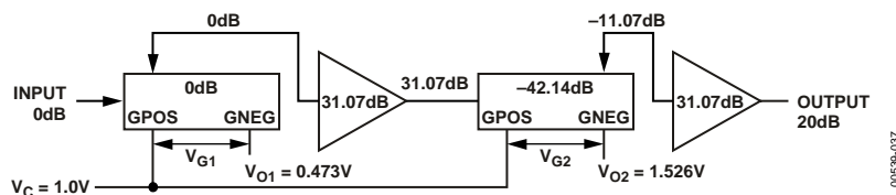
Figure 37. AD603 Gain Control Calculations for Sequential Control Operation V_C = 1.0\text{ V}
