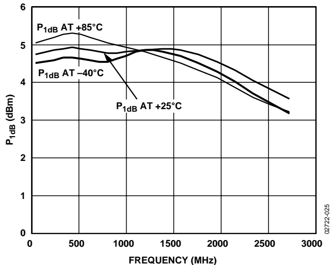
Figure 26. P_{1\text{dB}} vs. Frequency, V_S = 5\text{ V}, T_A = -40^\circ\text{C}, +25^\circ\text{C}, \text{ and } +85^\circ\text{C}
