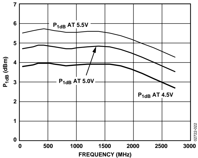
Figure 23. P_{1\text{dB}} vs. Frequency, V_S = 4.5\text{ V}, 5\text{ V}, \text{ and } 5.5\text{ V}, T_A = 25^\circ\text{C}
