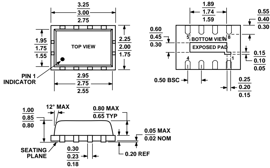
Figure 43. 8-Lead Lead Frame Chip Scale Package [LFCSP_VD] 2 mm x 3 mm Body, Very Thin, Dual Lead CP-8-1 Dimensions shown in millimeters
