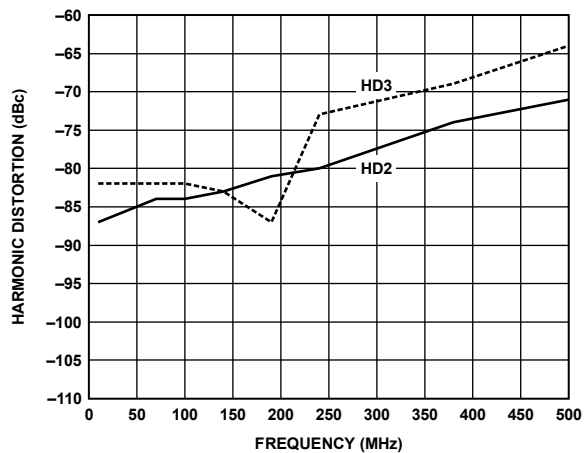
Figure 14. Harmonic Distortion vs. Frequency for 2 V p-p into R_L = 1 \text{ k}\Omega , A_V = 10 \text{ dB} , 5 V Supply, R_G = 180 \Omega , R_D = 6.8 \text{ k}\Omega , C_D = 0.1 \text{ pF}
