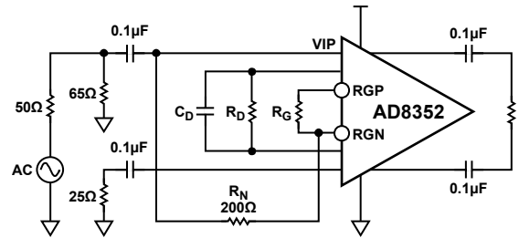
Figure 26. Single-Ended Schematic
