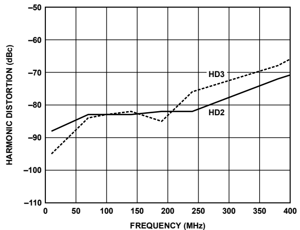
Figure 15. Harmonic Distortion vs. Frequency for 2 V p-p into R_L = 200 \Omega , A_V = 10 \text{ dB} , R_G = 115 \Omega , R_D = 4.3 \text{ k}\Omega , C_D = 0.2 \text{ pF}
