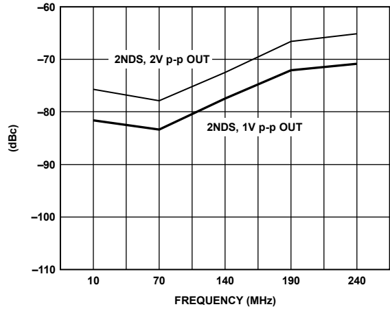
Figure 28. Single-Ended, Second-Order Harmonic Distortion, 200\ \Omega Load
