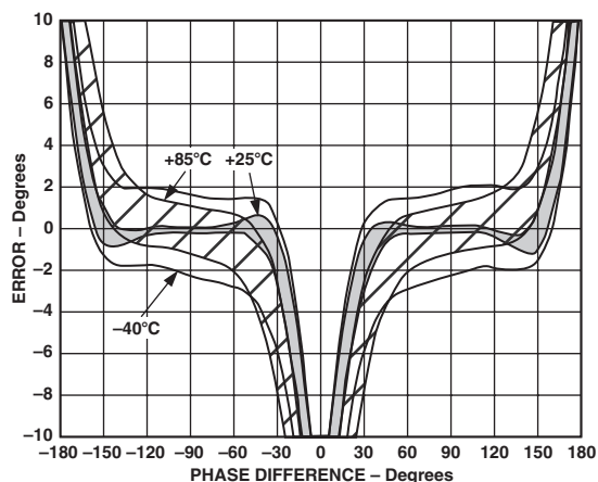
TPC 32. Distribution of VPBS Error vs. Input Phase Difference, Three Sigma to Either Side of Mean, Frequency 2200 MHz, -40°C, +25°C, and +85°C, Input Levels -30 dBm
