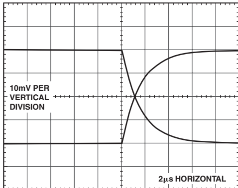
TPC 39. VPHS Output Response to 4° Step with Nominal Phase Shift of 90°, Input Levels P_{INPA} = P_{INPB} = -30 dBm, Supply 5 V, Frequency 1900 MHz, 25°C, with 100 pF Filter Capacitor
