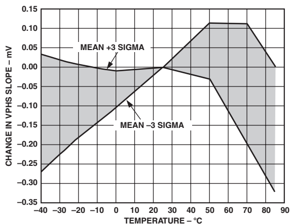
TPC 34. Change in VPBS Slope vs. Temperature, Three Sigma to Either Side of Mean, Frequency 1900 MHz
