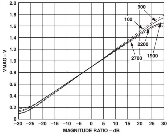
TPC 1. Magnitude Output (VMAG) vs. Input Level Ratio (Gain) V_{INPA}/V_{INPB} , Frequencies 100 MHz, 900 MHz, 1900 MHz, 2200 MHz, 2700 MHz, 25^\circ\text{C} , P_{INPB} = -30\text{ dBm} , (Re: 50\ \Omega )
