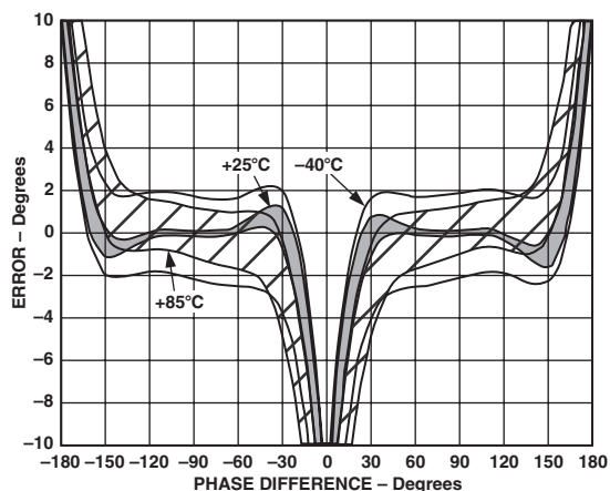
TPC 31. Distribution of VPBS Error vs. Input Phase Difference, Three Sigma to Either Side of Mean, Frequency 1900 MHz, -40°C, +25°C, and +85°C, Supply 5 V, Input Levels P_{INPA} = P_{INPB} = -30 dBm
