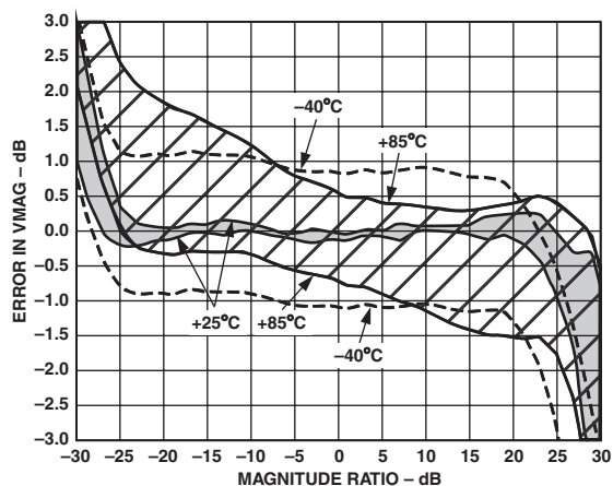
TPC 9. Distribution of Magnitude Error vs. Input Level Ratio (Gain), Three Sigma to Either Side of Mean, Temperatures -40^{\circ}\text{C} , +25^{\circ}\text{C} , and +85^{\circ}\text{C} , Reference Level = -30\text{ dBm}
