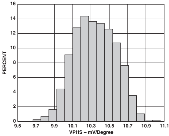
TPC 37. VPHS Slope Distribution, Frequency 900 MHz
