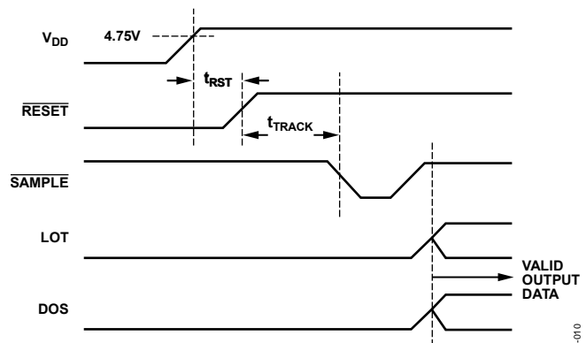
Figure 10. Power Supply Sequencing and Reset
