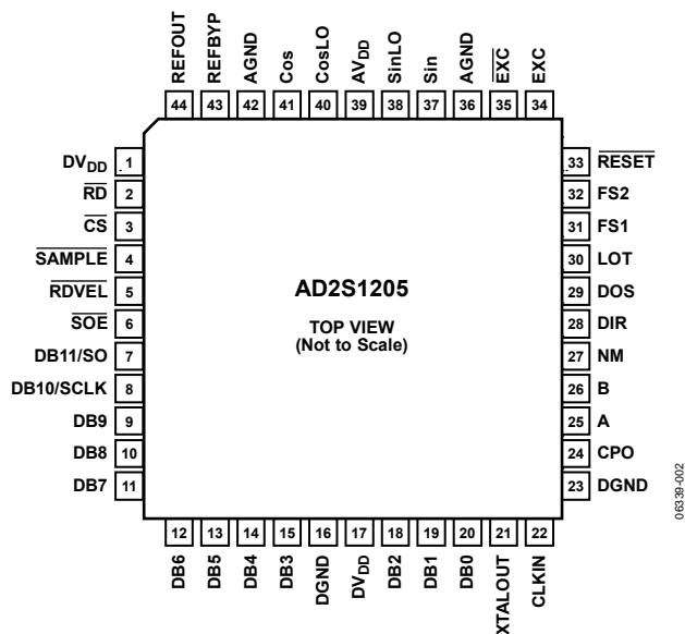
Figure 2. Pin Configuration
