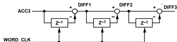
Figure 27. Differentiator
