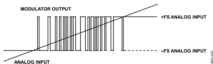
Figure 21. Analog Input vs. Modulator Output
