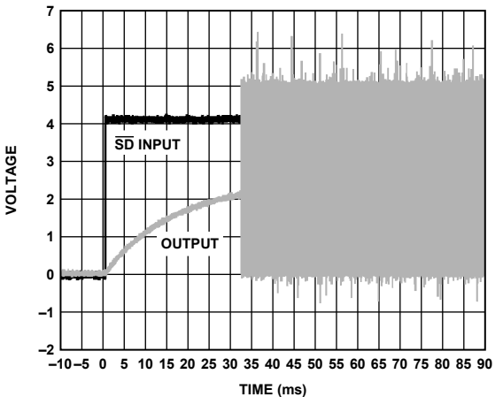
Figure 35. Turn-On Response
