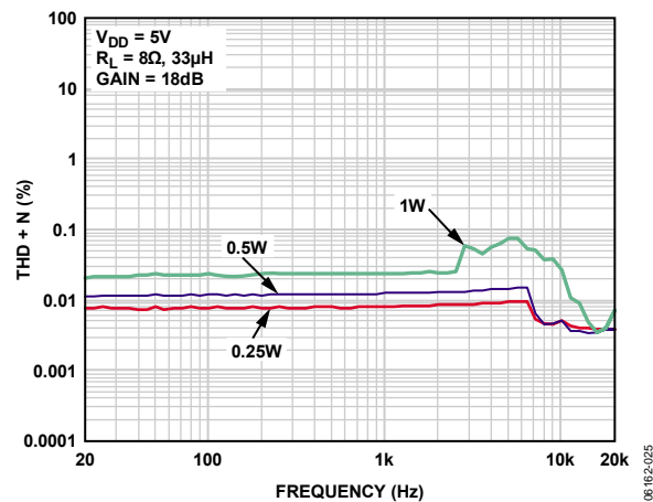
Figure 13. THD + N vs. Frequency, V_{DD} = 5V , R_L = 8\Omega , A_V = 18dB
