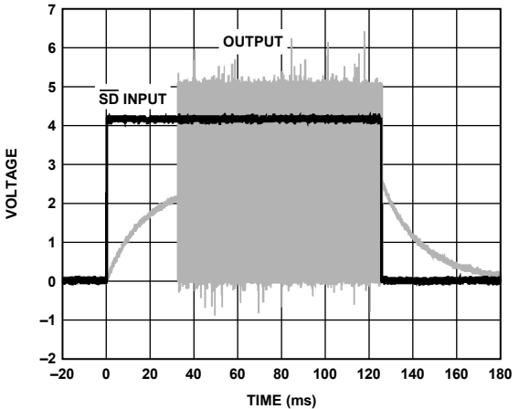
Figure 36. Turn-Off Response
