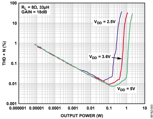
Figure 4. THD + N vs. Output Power into 8 \Omega , A_v = 18 dB
