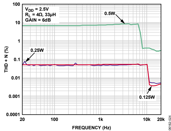
Figure 12. THD + N vs. Frequency, V_{DD} = 2.5V , R_L = 4\Omega , A_V = 6dB
