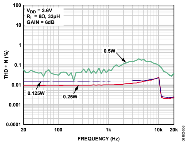
Figure 8. THD + N vs. Frequency, V_{DD} = 3.6 V, R_L = 8 \Omega , A_v = 6 dB
