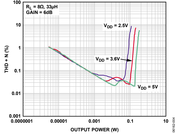
Figure 6. THD + N vs. Output Power into 8 \Omega , A_v = 6 dB
