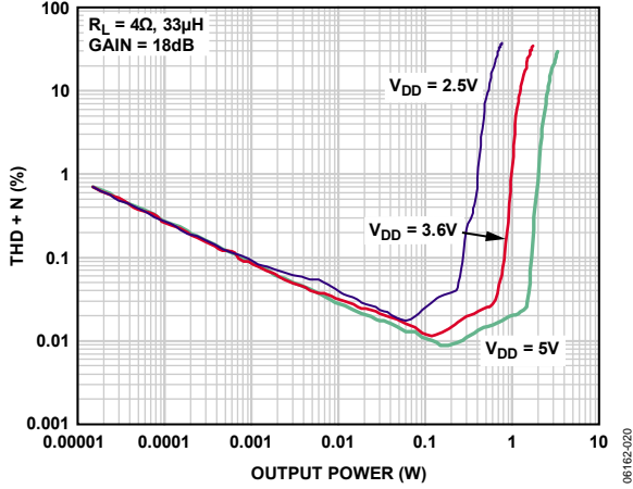
Figure 3. THD + N vs. Output Power into 4 \Omega , A_v = 18 dB
