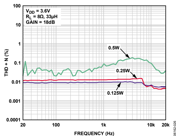
Figure 14. THD + N vs. Frequency, V_{DD} = 3.6V , R_L = 8\Omega , A_V = 18dB
