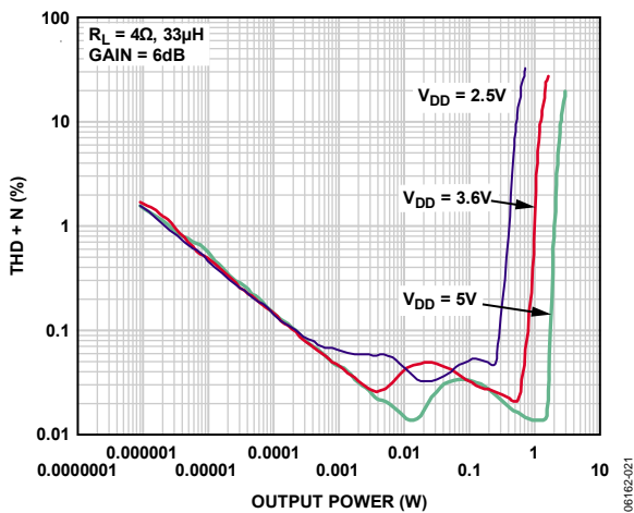
Figure 5. THD + N vs. Output Power into 4 \Omega , A_v = 6 dB
