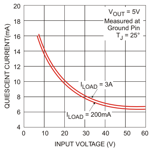
Figure 5. Quiescent Current
