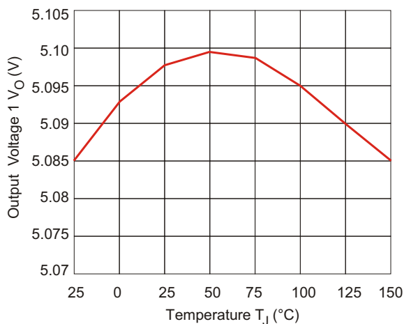
Figure 6. Output Voltage1 vs. Temperature
