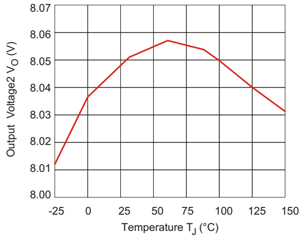
Figure 7. Output Voltage2 vs. Temperature( T_J )
