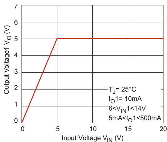
Figure 2. Output Voltage 1 vs. Input Voltage
