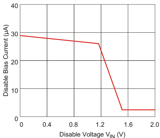
Figure 5. Disable Bias Current vs. e Voltage
