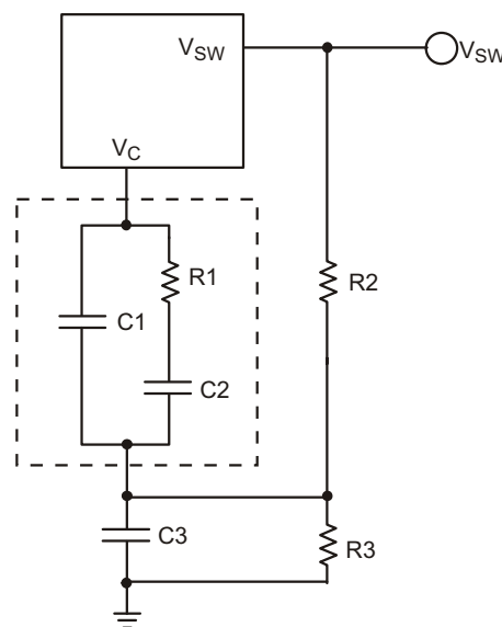
Figure 14. Technique for Increasing Slope Compensation
