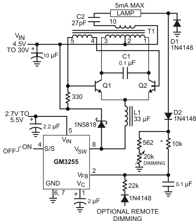
Figure 27. CCFL Supply
