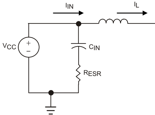
Figure 11. Boost Circuit Effective Input Filter
