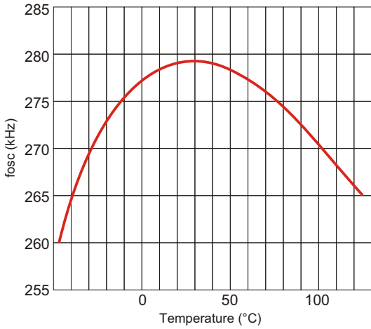
Figure 3. Switching Frequency vs. Temperature (GM3255 only)
