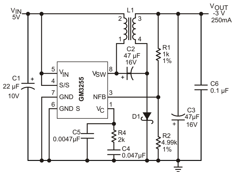
Figure 26. Low Ripple 5V to -3V "Cuk" Converter
