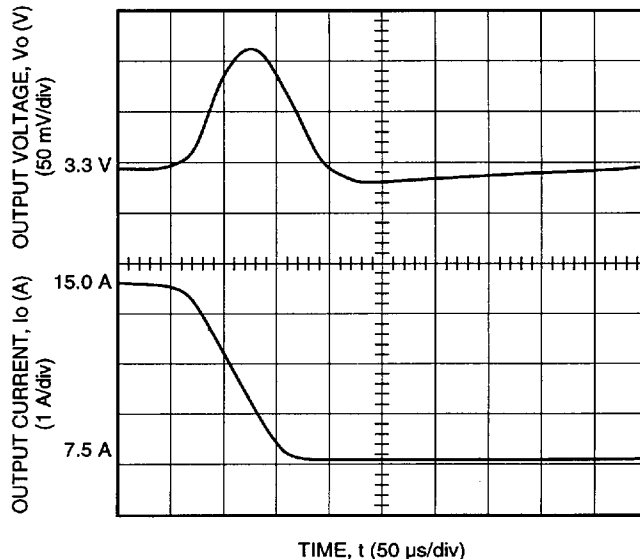
Figure 15. Typical JW150F Transient Response to Step Decrease in Load from 50% to 25% of Full Load at Room Temperature and 48 V Input (Waveform Averaged to Eliminate Ripple Component.)
