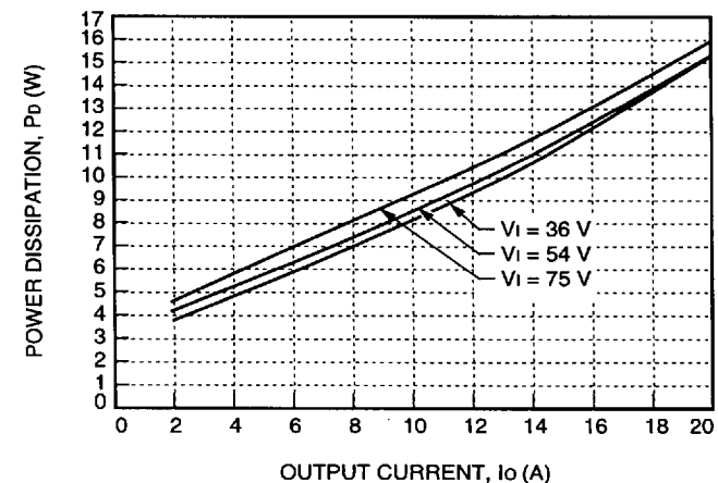
Figure 29. JW100F Power Dissipation vs. Output Current
