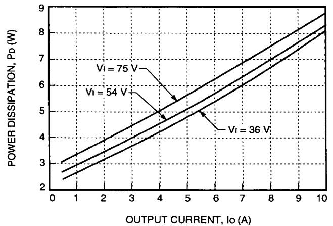
Figure 27. JW050F Power Dissipation vs. Output Current
