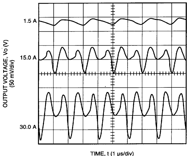
Figure 13. Typical JW150F Output Ripple Voltage at Room Temperature, 48 V Input, I_o = Full Load
