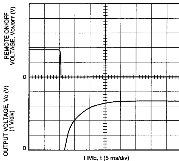
Figure 16. Typical Start-Up from Remote On/Off JW150F1; I_o = Full Load
