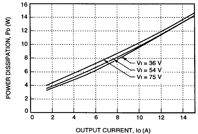
Figure 28. JW075F Power Dissipation vs. Output Current
