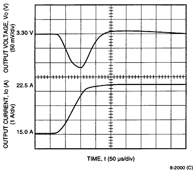
Figure 14. Typical JW150F Transient Response to Step Increase in Load from 50% to 75% of Full Load at Room Temperature and 48 V Input (Waveform Averaged to Eliminate Ripple Component.)
