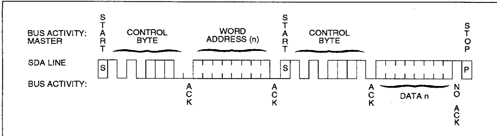
FIGURE 9-2: RANDOM READ
