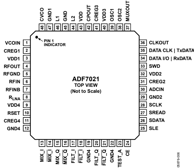
Figure 6. Pin Configuration
