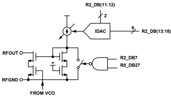
Figure 14. PA Configuration in FSK/GFSK Mode
