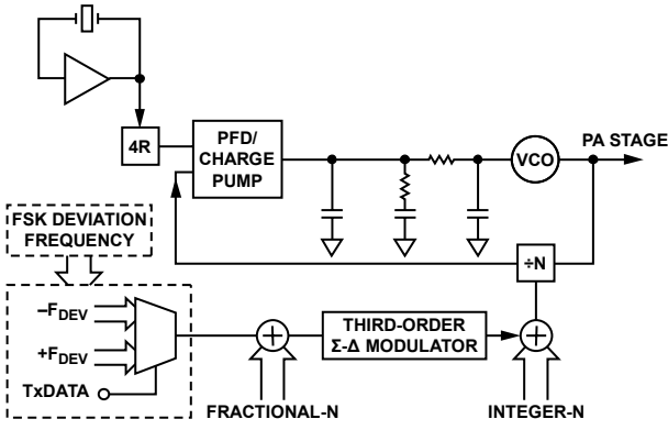
Figure 16. 2FSK Implementation
