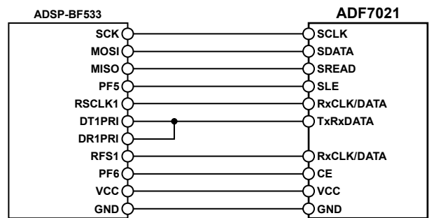
Figure 29. ADSP-BF533 to ADF7021 Connection Diagram
