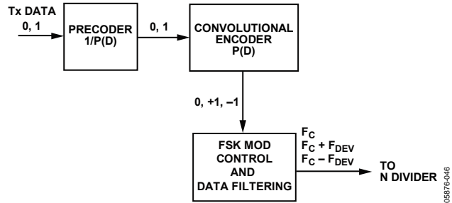
Figure 17. 3FSK Encoding
