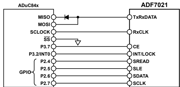
Figure 28. ADuC84x to ADF7021 Connection Diagram
