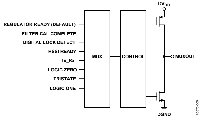
Figure 11. MUXOUT Circuit
