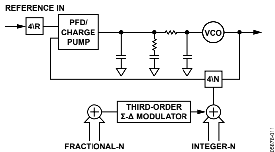
Figure 10. Fractional-N PLL
