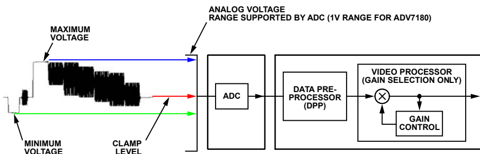
Figure 25. Gain Control Overview
