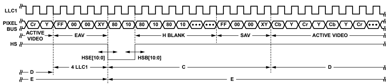
Figure 32. HS Timing
