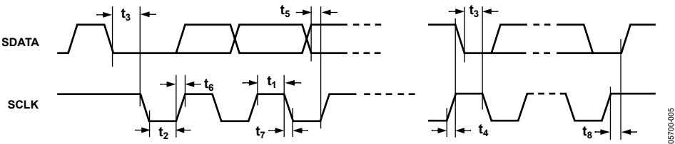
Figure 5. I²C Timing
