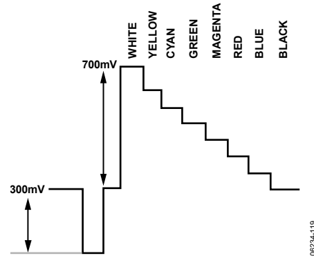
Figure 119. Y Levels—PAL
