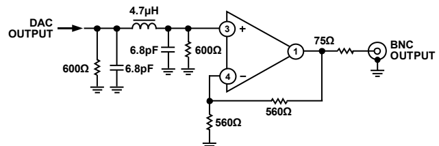
Figure 87. Example of Output Filter for ED, 8x Oversampling
