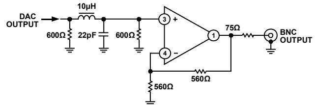
Figure 86. Example of Output Filter for SD, 16x Oversampling
