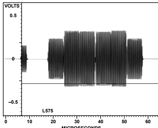
Figure 134. PAL Luma
