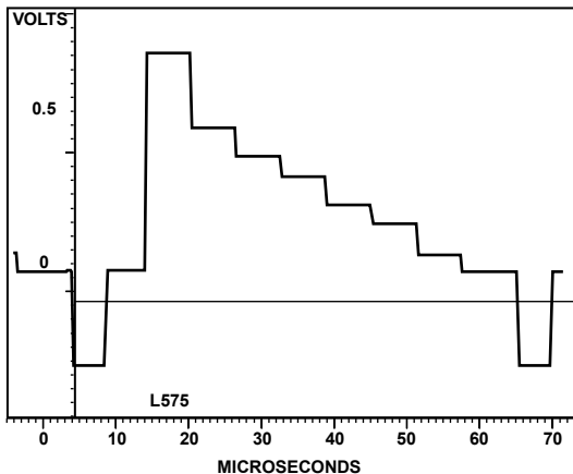
Figure 134. PAL Luma
