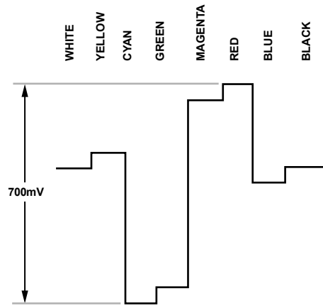
Figure 120. Pr Levels—PAL
