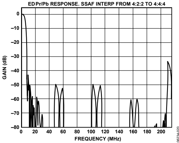
Figure 20. ED 8x Oversampling, PrPb Filter (SSAF) Response
