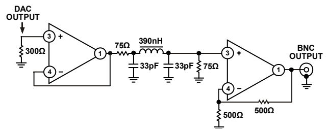
Figure 88. Example of Output Filter for HD, 4x Oversampling
