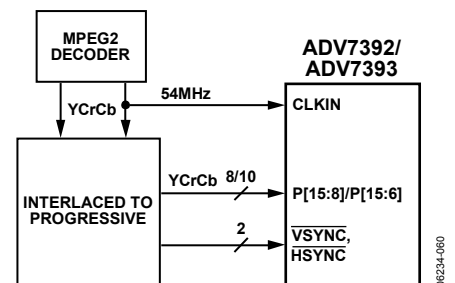
Figure 60. ED (At 54 MHz) Example Application
