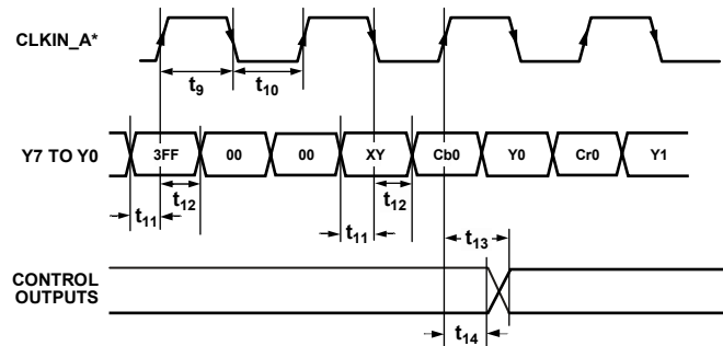
Figure 9. ED/HB-DDR Only, 8-Bit, 4:2:2 YCrCb (EAV/SAV) Pixel Input Mode (Input Mode 010)
