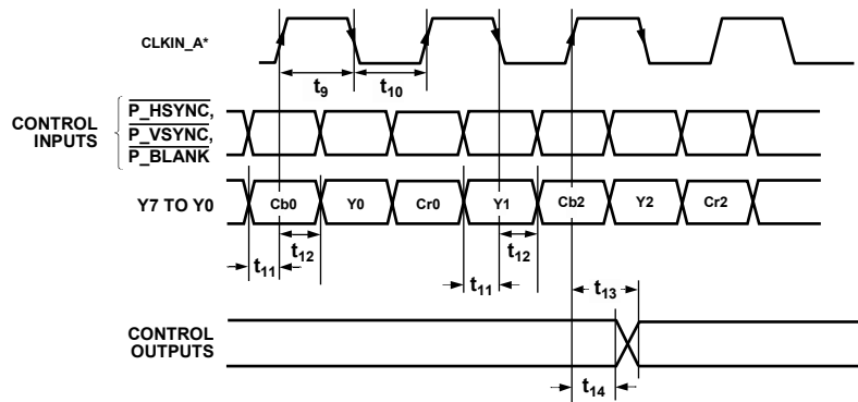
Figure 8. ED/HB-DDR Only, 8-Bit, 4:2:2 YCrCb (HSYNC/VSYNC) Pixel Input Mode (Input Mode 010)
