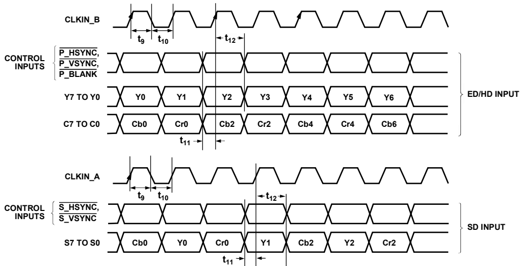
Figure 10. SD and ED/HB-SDR, 16-Bit, 4:2:2 ED/HB and 8-Bit, SD Pixel Input Mode (Input Mode 011)
