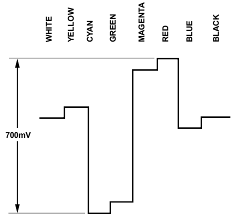
Figure 118. Pr Levels—PAL
