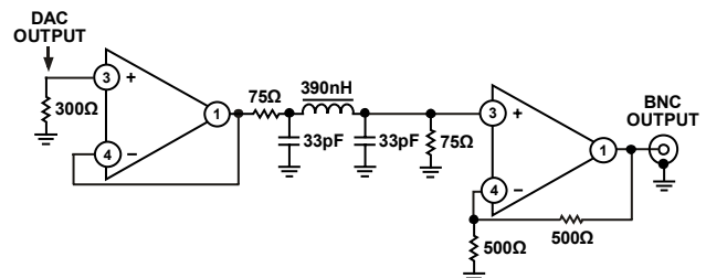
Figure 86. Example of Output Filter for HD, 4× Oversampling
