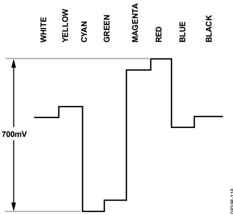
Figure 115. Pr Levels—NTSC
