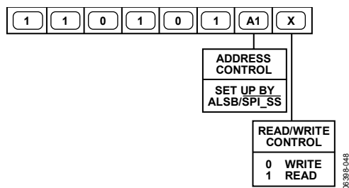
Figure 48. ADV7340 Slave Address = 0xD4 or 0xD6
