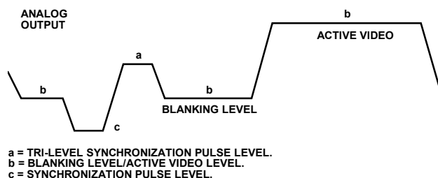
Figure 59. ED/HD Nonstandard Timing Mode Output Levels
