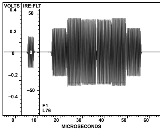
Figure 129. NTSC Luma
