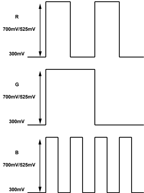
Figure 124. SD/ED RGB Output Levels—RGB Sync Disabled
