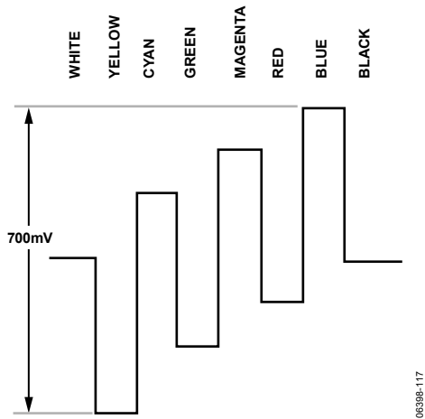
Figure 116. Pb Levels—NTSC
