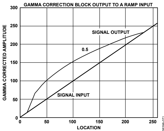
Figure 70. Signal Input (Ramp) and Signal Output for Gamma 0.5
