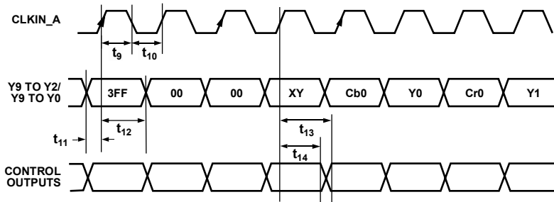
Figure 13. ED Only (at 54 MHz), 8-/10-Bit, 4:2:2 YCrCb (EAV/SAV) Pixel Input Mode (Input Mode 111)
