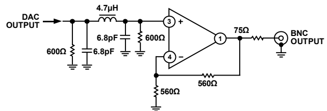
Figure 85. Example of Output Filter for ED, 8× Oversampling
