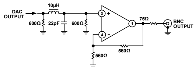
Figure 84. Example of Output Filter for SD, 16× Oversampling
